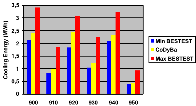
Fig. R11 : High Mass Annual Cooling
