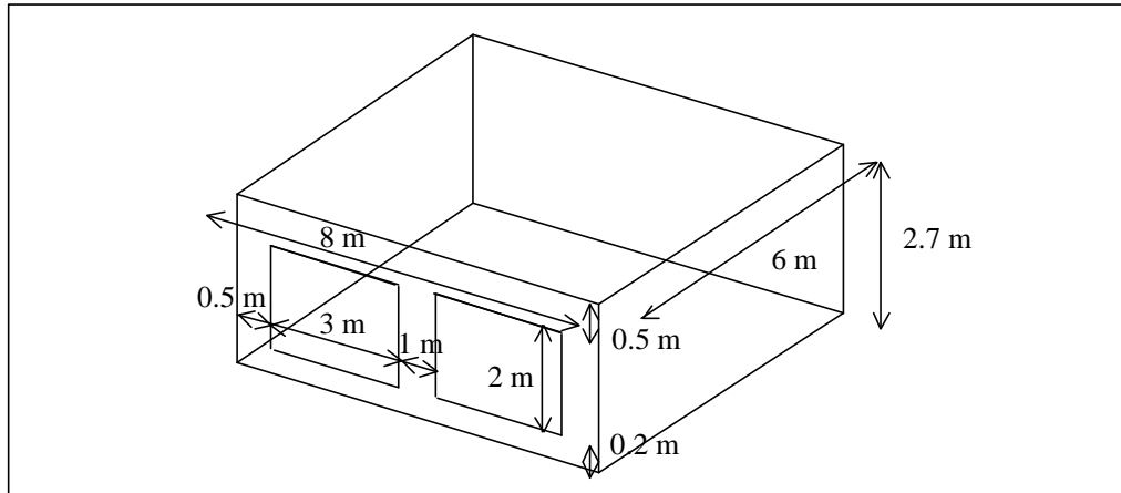
Figure A : south unshaded window building
